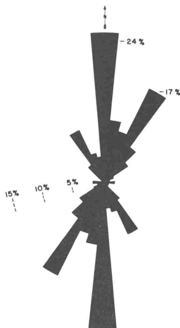
Fig. 18—Fault-strike frequency diagrams for areas in the Great Basin of western United States. (a) Strikes of 625 faults or fault segments plotted at 1-degree intervals. Radius of diagram equals 18 faults or fault segments. (b) Same data replotted for 5-degree class intervals. Radius of diagram equals 62 faults or fault segments (from Donath, Ref. 86, Fig. 4). (c) Strikes of 410 range-edges in over 50,000 sq mi in Nevada, as measured from 1:250,000 USGS topographic sheets (from Conger, Ref. 91).
